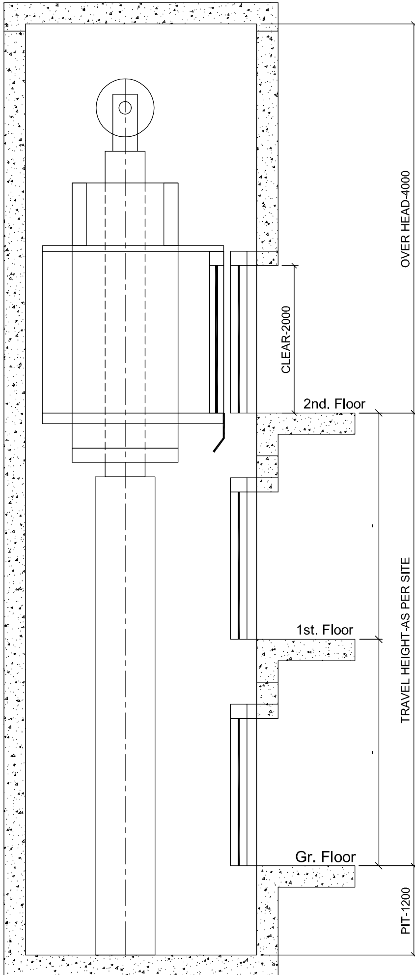
LIFT WELL SECTION VIEW
